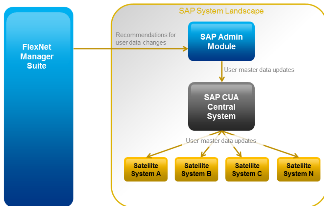
Figure 5: Data flow from FlexNet Manager Suite to the SAP systems when using CUA
